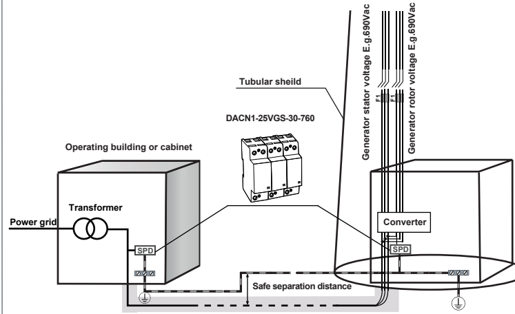
Fig. Double-fed induction asynchronous generator(DFIG)application
